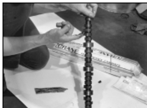
Figure 3. Apply lots of assembly lube to each cam lobe as shown.
